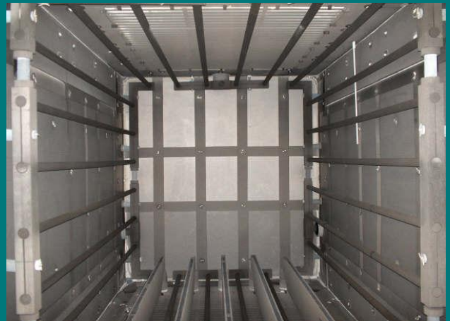
"Hot zone rebuild of an over pressure quench vacuum furnace"
